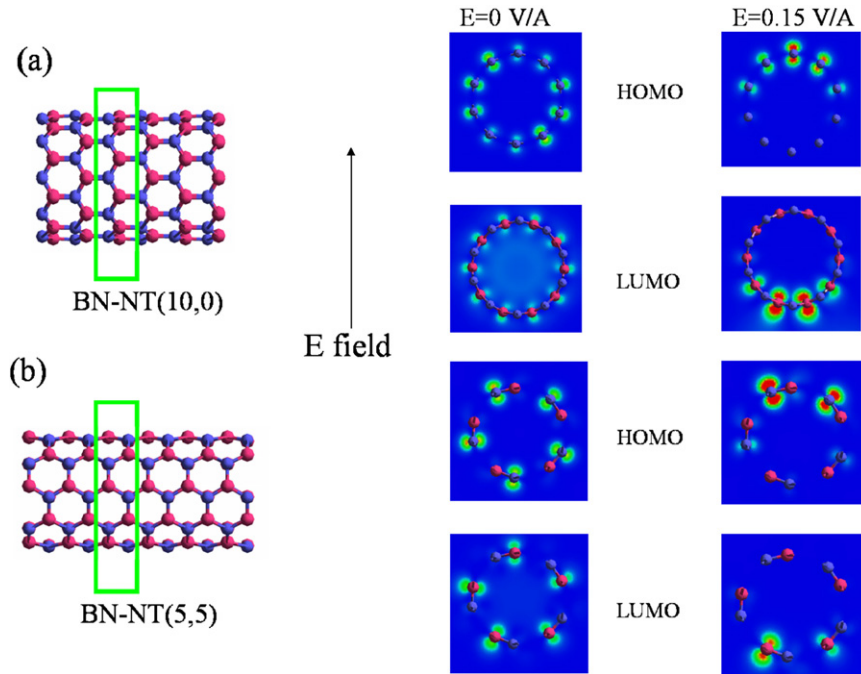
Figure 6. Charge redistribution in the VBM and CBM states for (a) (10, 0) and (b) (5, 5) BN-NTs under an external electric field of 0 and 0.15 V Å -1 , respectively.
