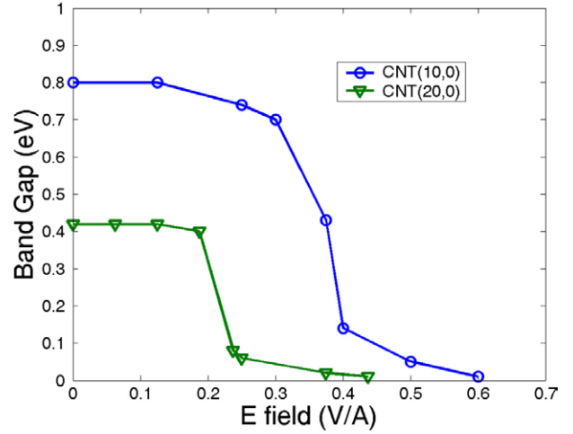
Figure 2. The band gaps of (10, 0) and (20, 0) CNTs as a function of field strength.
