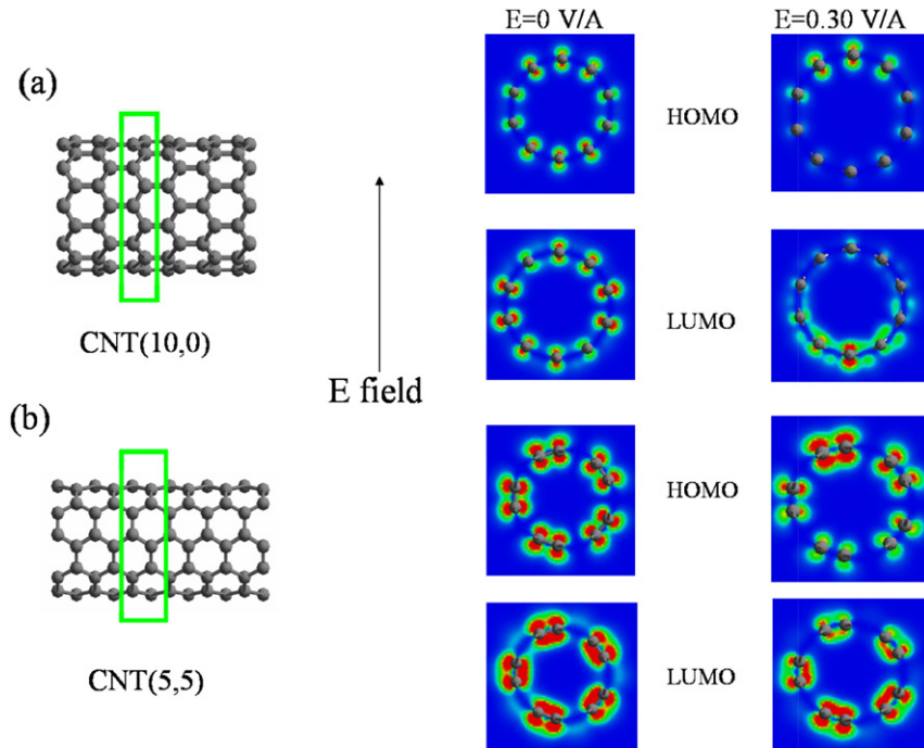
Figure 5. Charge redistribution in the VBM and CBM states for (a) (10, 0) and (b) (5, 5) CNTs under an external electric field of 0 and 0.30 \text{ V } \text{\AA}^{-1} , respectively.
