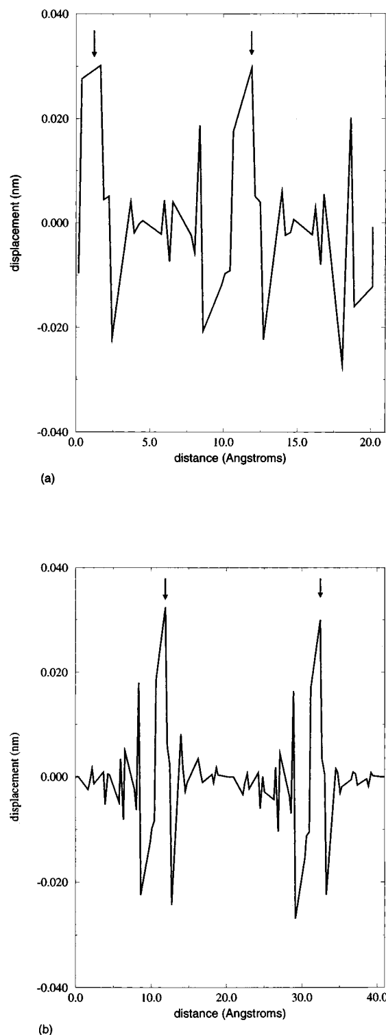
FIG. 2. Differential displacements normal to the boundary plane of the oxygen sublattice atomic layers for (a) the 60-atom model and (b) the 120-atom model. The arrows indicate the locations of the two boundaries in the models. Note the difference in the horizontal scales for (a) and (b).
