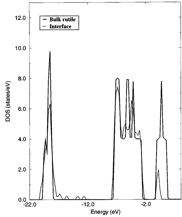
FIG. 7. Total normalized valence band density of states (DOS) at (\frac{1}{4}, 0, \frac{1}{4}) for bulk rutile and the relaxed 60-atom supercell. Note the increased bandwidth in the boundary system. This is consistent with the overall trend towards bond length reduction in the boundary core. A decrease in bond length means that the atoms are pushed closer together, i.e., there is greater orbital overlap than in the bulk, hence a larger bandwidth. The band gap is from -2.9 to -0.3 eV.
