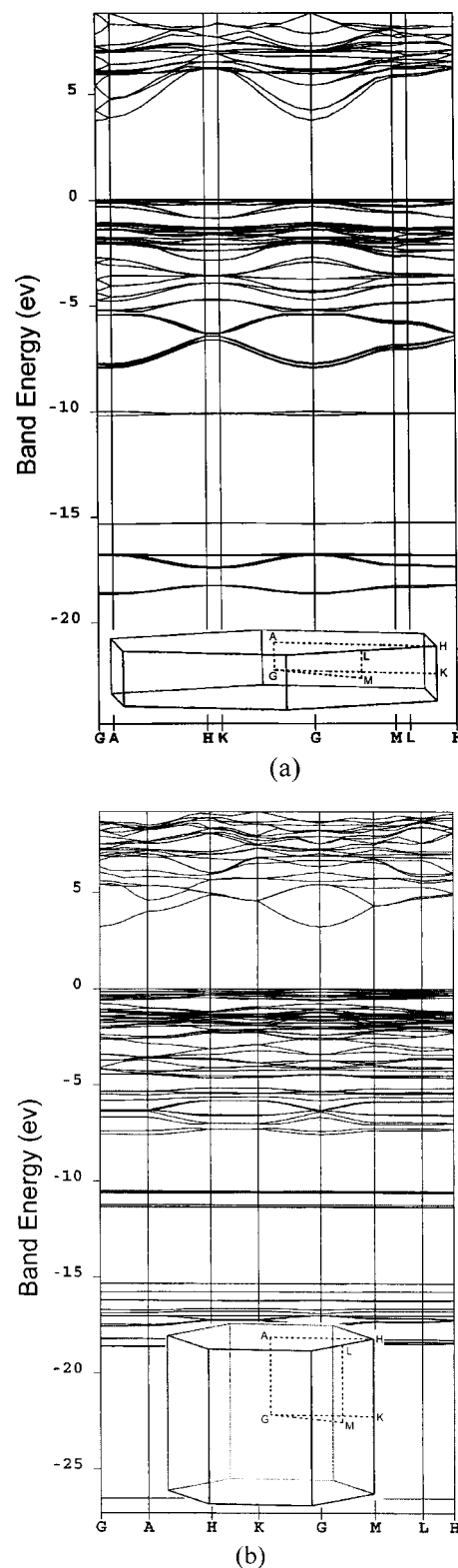
FIG. 2. Band structure of BABO and KABO: (a) BABO and (b) KABO.
