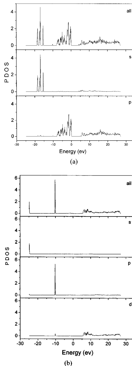
FIG. 4. Orbital resolved PDOS plot for BABO: (a) O and (b) Ba.
