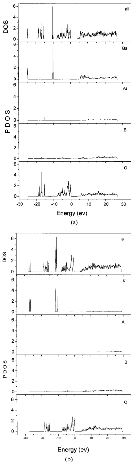
FIG. 3. DOS and PDOS plots of BABO and KABO: (a) BABO and (b) KABO.
