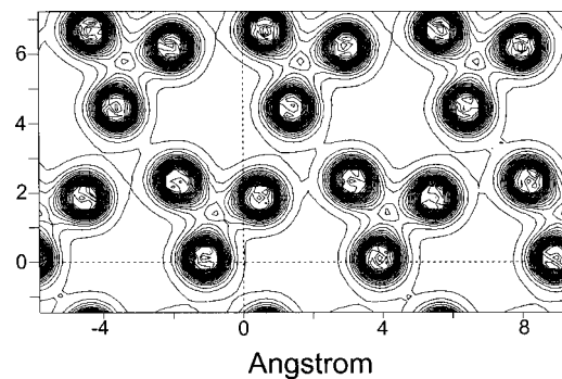
FIG. 6. Charge density in the (\text{BO}_3)^{3-} group plane of BABO.
