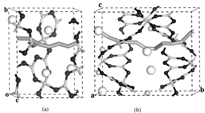
FIG. 3. (Color online) The representative results for the diffusion of a water molecule in CBO and CLBO crystals. The green lines denote the diffusion path of \text{H}_2\text{O} along the a axis in a CBO crystal (a), and along the b axis in a CLBO crystal (b).
