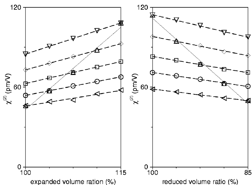
FIG. 4. Original (solid lines) and “equal-gap” re-evaluated (dashed lines) \chi^{(2)} of AgGaS 2 (left panel) and AgGaSe 2 (right panel). For those five cell volumes marked with the same symbol (dashed line), their band gaps are adjusted to be identical for evaluating \chi^{(2)} . Significant reduction of the slope indicates that the band gap has to play an important role in \chi^{(2)} variation, while the reminding slope suggests the existence of other factor(s).
