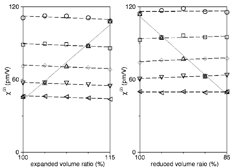
FIG. 6. The original \chi^{(2)} of AgGaS 2 (left panel) and AgGaSe 2 (right panel), are shown alone fitted solid lines, while the fitted dashed lines emphasize the re-evaluated \chi^{(2)} of those crystals with different cell volumes but using the same energy level spacing from only one of the crystals. One can see that these dashed line are much flatter than the original solid lines. This indicates the effect of energy level spectra solely controls the \chi^{(2)} in these crystals.
