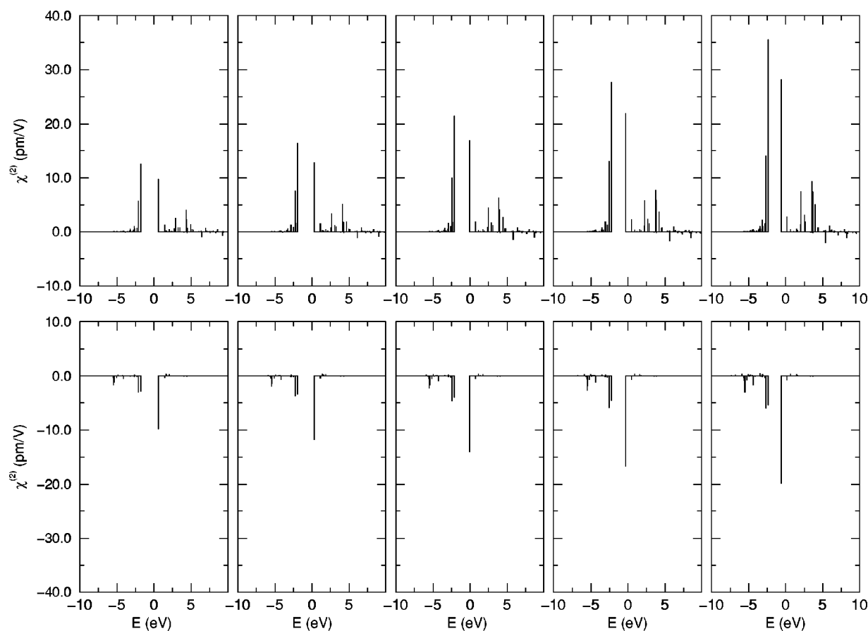
FIG. 5. Band-resolved \chi^{(2)} of AgGaS 2 at zone center. The upper row are the virtual electron contributions and the lower row are the virtual hole ones. The five cell volumes are displayed from left to right, corresponding to the uniform expansion from 100% to 115%. One can see that these “densities of \chi^{(2)} ” share the same pattern, also the energy level spacing reduces with respect to the increase of cell volume. (Note that in each plot, summing up all the peaks on the left to the band gap will get same value as summing up all the peaks to the right, which is equal to the \chi^{(2)} of that process.) In this material, the virtual electron process is more important than virtual hole processes, and they are in opposite directions so they have a cancellation effect. Other k points show the same behavior but the magnitude is smaller. The results of AgGaSe 2 are similar to those of AgGaS 2 and are therefore not shown here.
